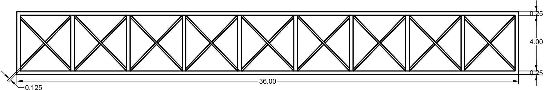
BOTTOM VIEW
