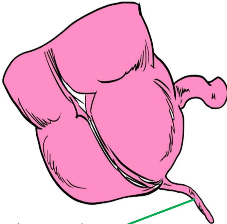
Normal Appendicitis
