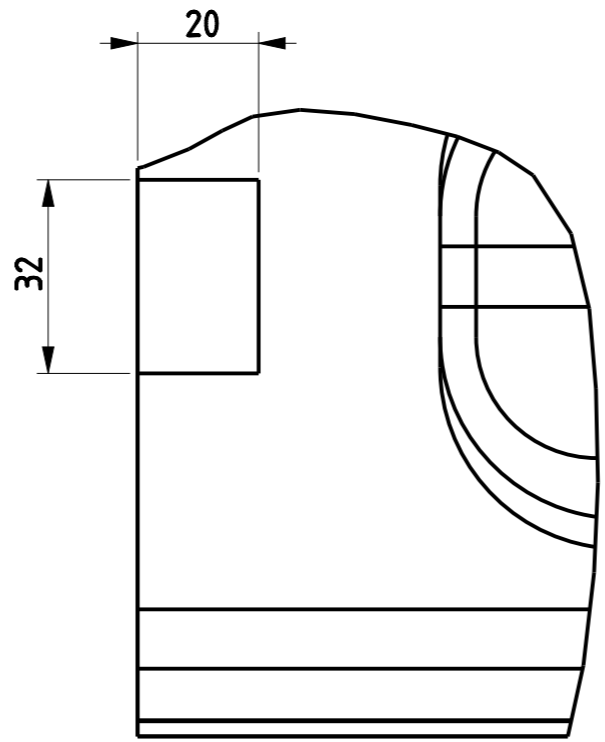
WIREFRAME VIEW SHOWING CUTOUT NOTCH - DETAIL B SCALE 0,800
