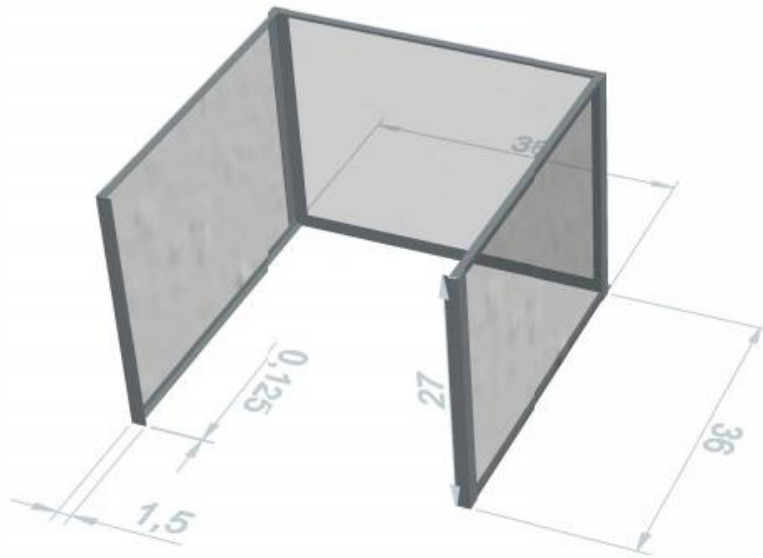
Figure 5.6 AutoCAD model displaying dimensions of barrier and aluminum angle bars (Created by Molly Milford)
