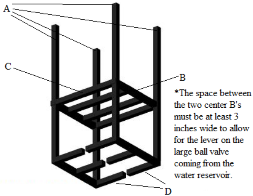
Figure F-4: Top angled view (Zirkel).
