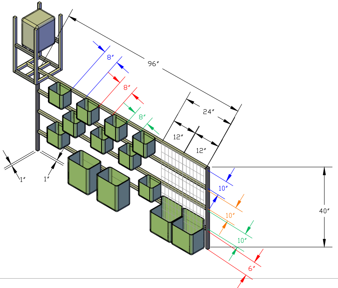
Figure F-1: The dimensions of one 8-foot section of Life Support (Trejo).
