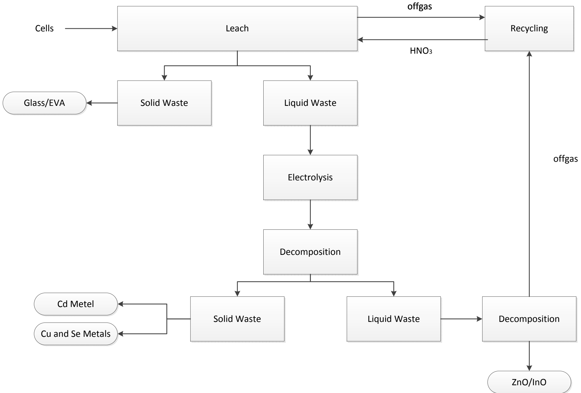
Chemical Recycling Process
