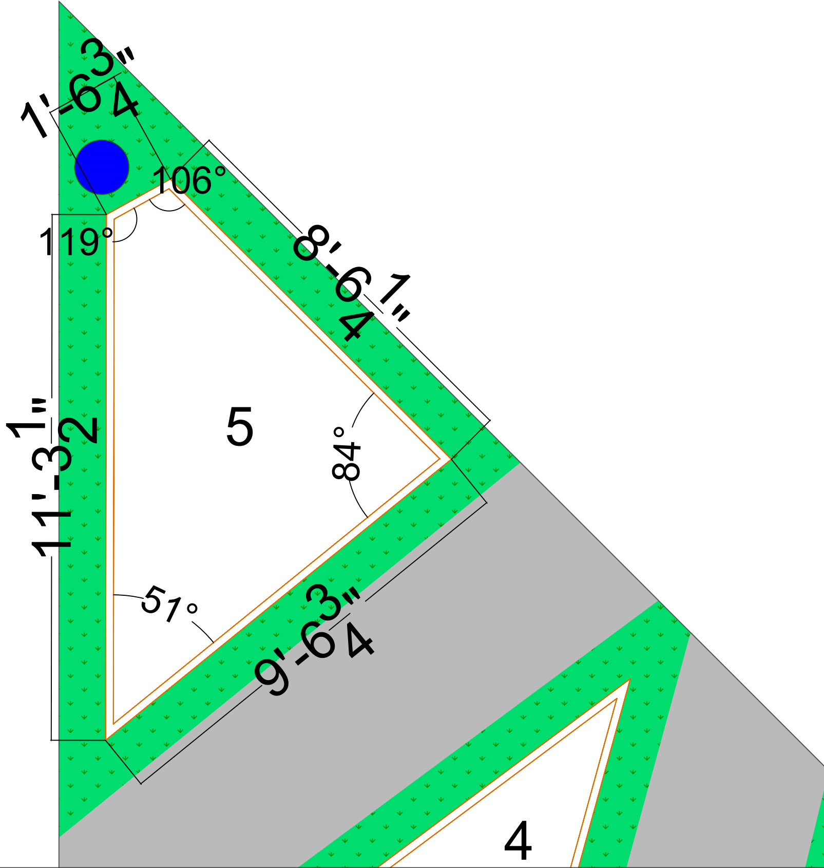
Top View of Planter 5
