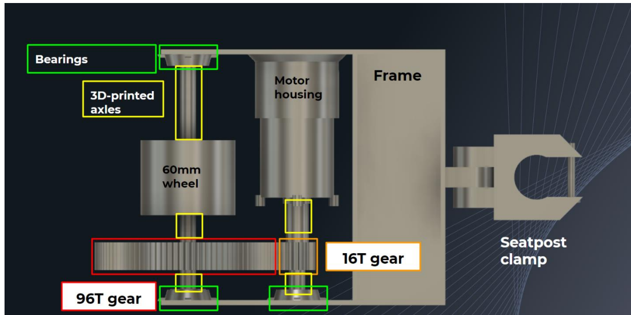
Figure 5-10 Renderings of all components in their respective final places
