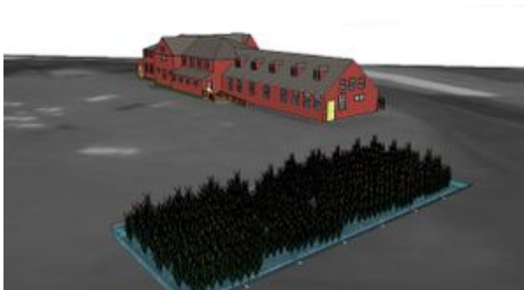
Figure 27: Secondary treatment horizontal constructed wetland: (“Samoa Hostel grey water island” 2013)
