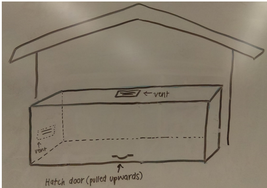
Figure 313 The No Chill Hatch is a single unit box that has a hatch door in the front, a triangle roof for cover and no method of refrigeration. A vent is located on the top and side of the unit for ventilation.
