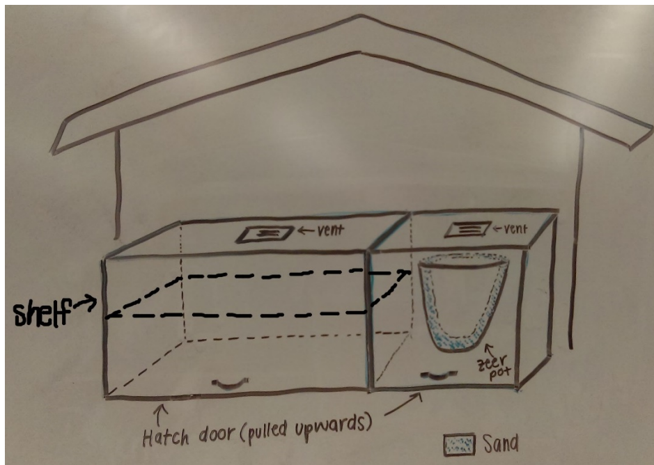
Figure 312 Pot o' Gold is a two-compartment box that uses the zeer pot refrigeration method, has hatch doors in the front, and has a triangle roof for cover. A vent is located on top of both compartments for ventilation.
