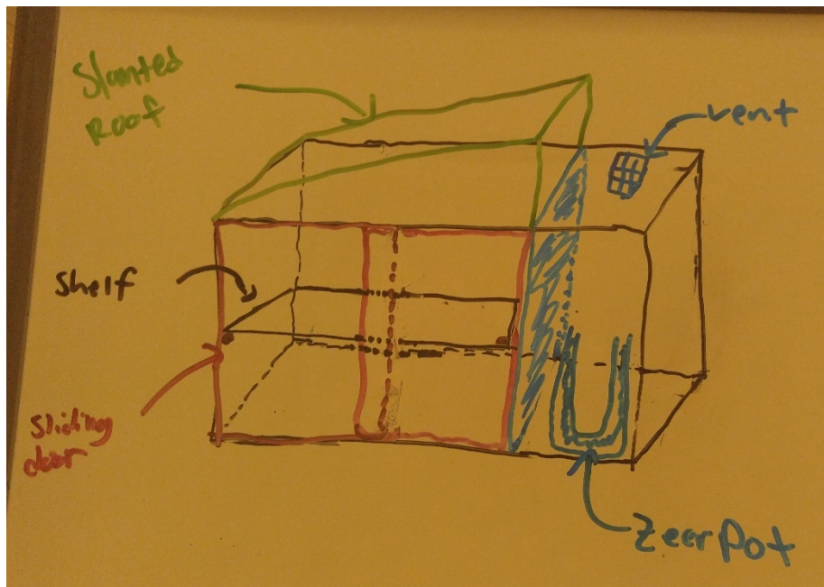
Figure 36 The Zeer Slider is a two-compartment box that uses the zeer pot refrigeration method, has sliding doors in the front, and has a slanted roof for cover. A vent is located on top of the zeer pot compartment for ventilation.
