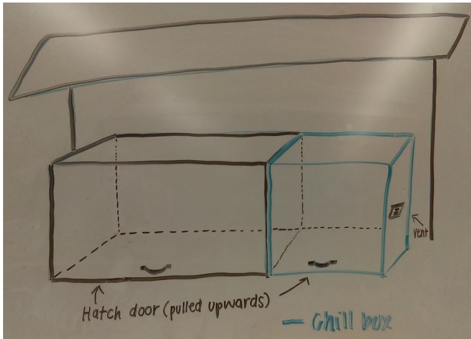
Figure 311 The Chill Hatch is a two-compartment box that uses the chill box refrigeration method, has hatch doors in the front, and has a slanted roof for cover. A vent is located on the side of the chill box compartment for ventilation.
