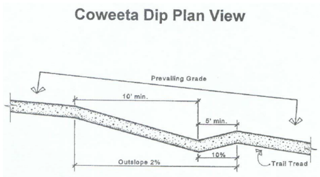
Figure 3-7 Coweeta Dip construction diagram (U.S. Department of the Interior 1996)
