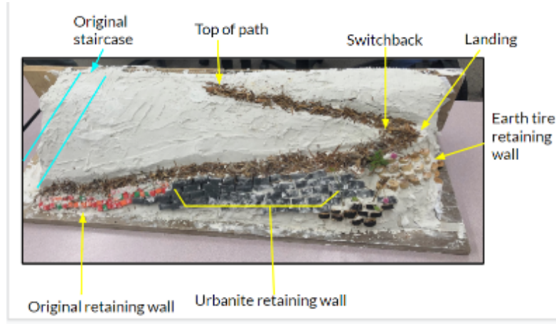
Figure 5-6 Prototype 1
