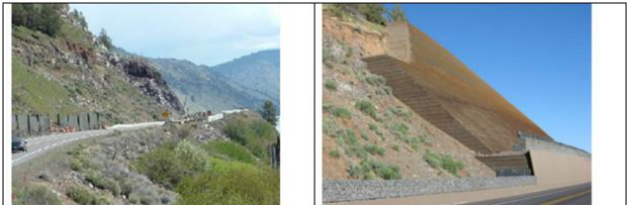
Figure 3-10 Before/after of US 97: Modoc Point - Hagelstein Park Project (Hilfiker Retaining Walls 2015)
