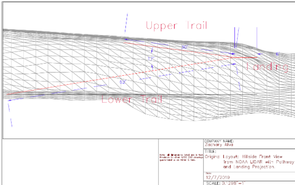
Figure 5-2 Final trail design - east facing view (Alva 2019)
