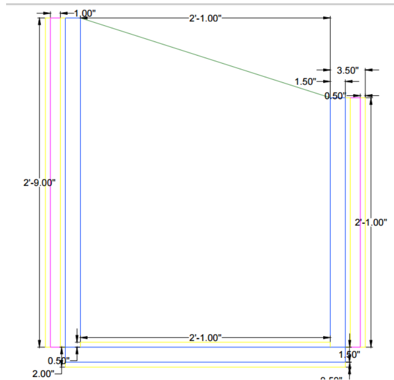
Figure 5-2 A side view of the upper cabinet that includes thickness, length and height dimensions
