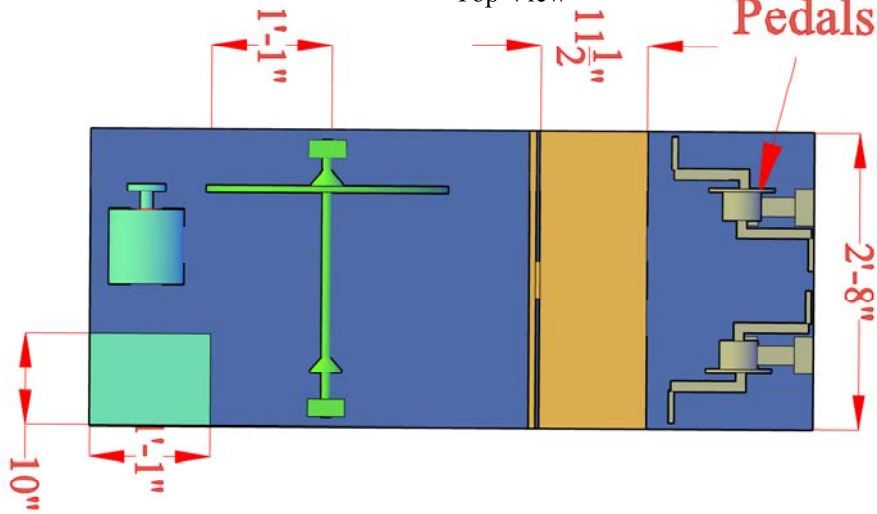
Shelving unit housing inverter/battery/blender Top View
